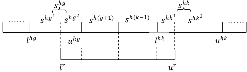
Figure 4.5: Method of converting Case 2 to Case 1
