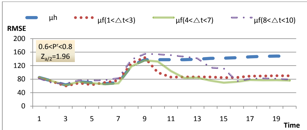
Figure 6.4: Sensitivity analysis for time delay
