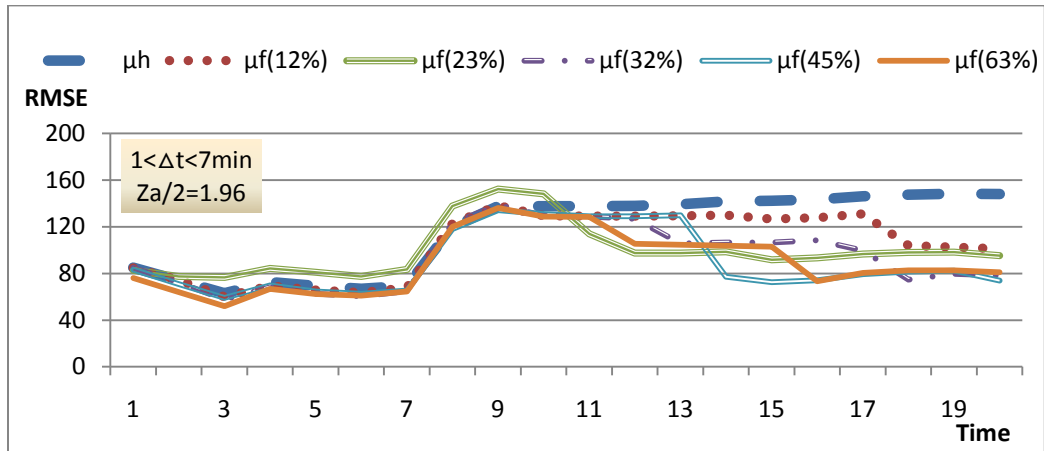
Figure 6.6: Sensitivity analysis for good information rate
