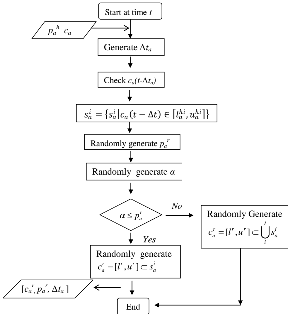
Figure 5.2: Semi-random procedure: generate real-time information
