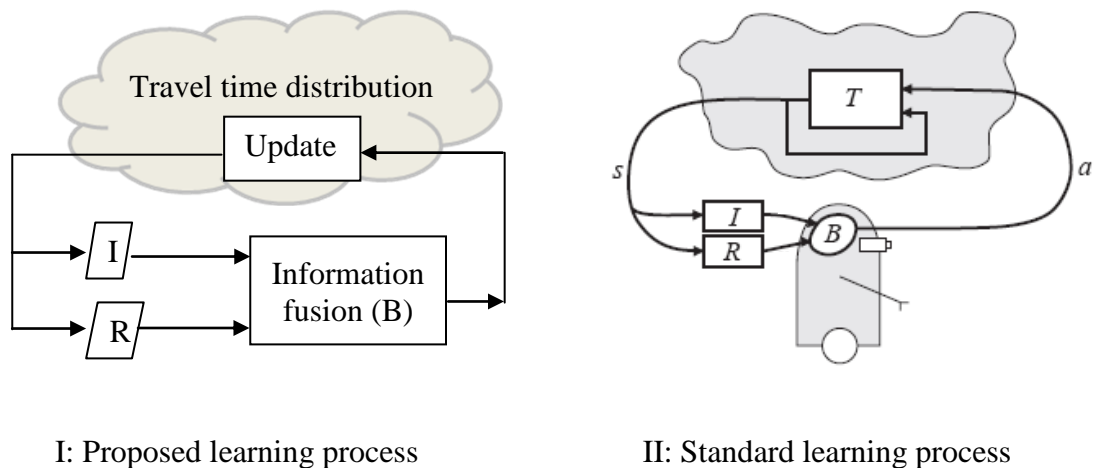
Figure 4.1: The proposed learning process and standard reinforcement learning
