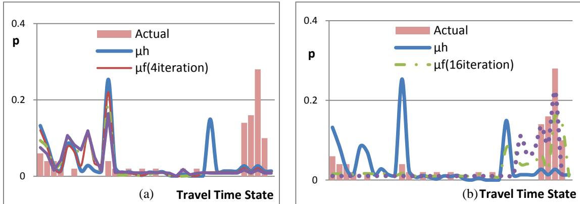
Figure 6.1: Travel time distributions on a link
