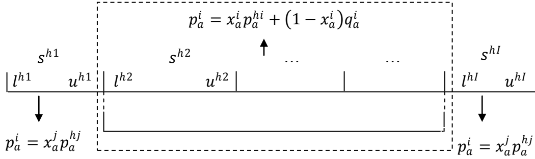
Figure 4.3: Information fusion model for Case 1
