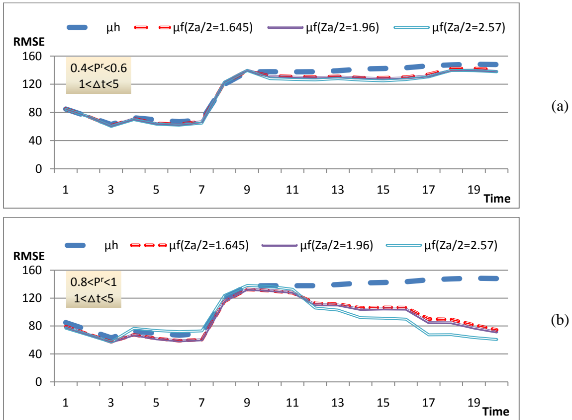
Figure 6.5: Sensitivity analysis for significance level
