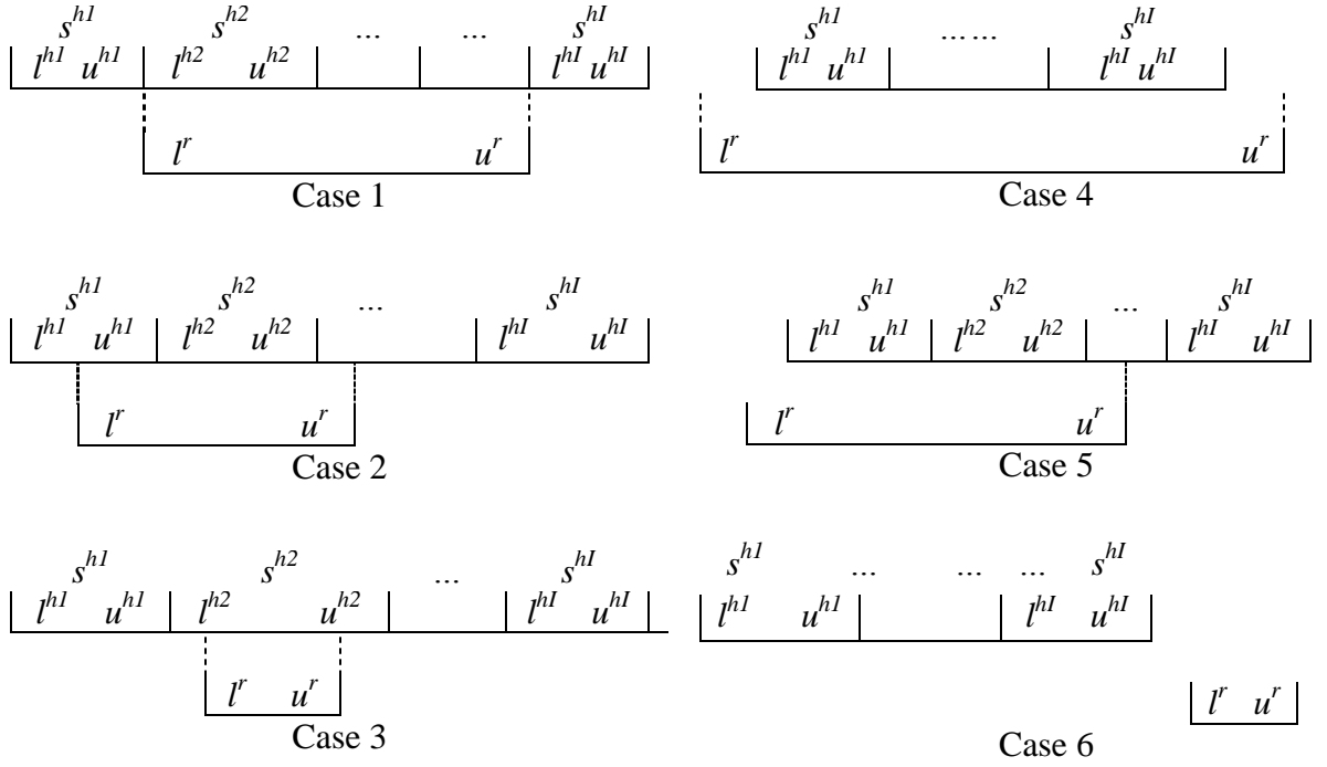
Figure 4.2: The relationship between the historical travel time distribution and the real-time travel time information
