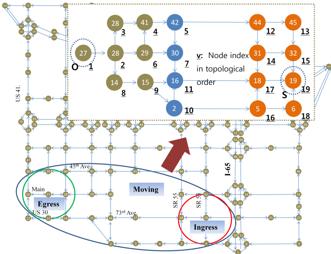
Figure 7.1: The DAG used in online stochastic routing
