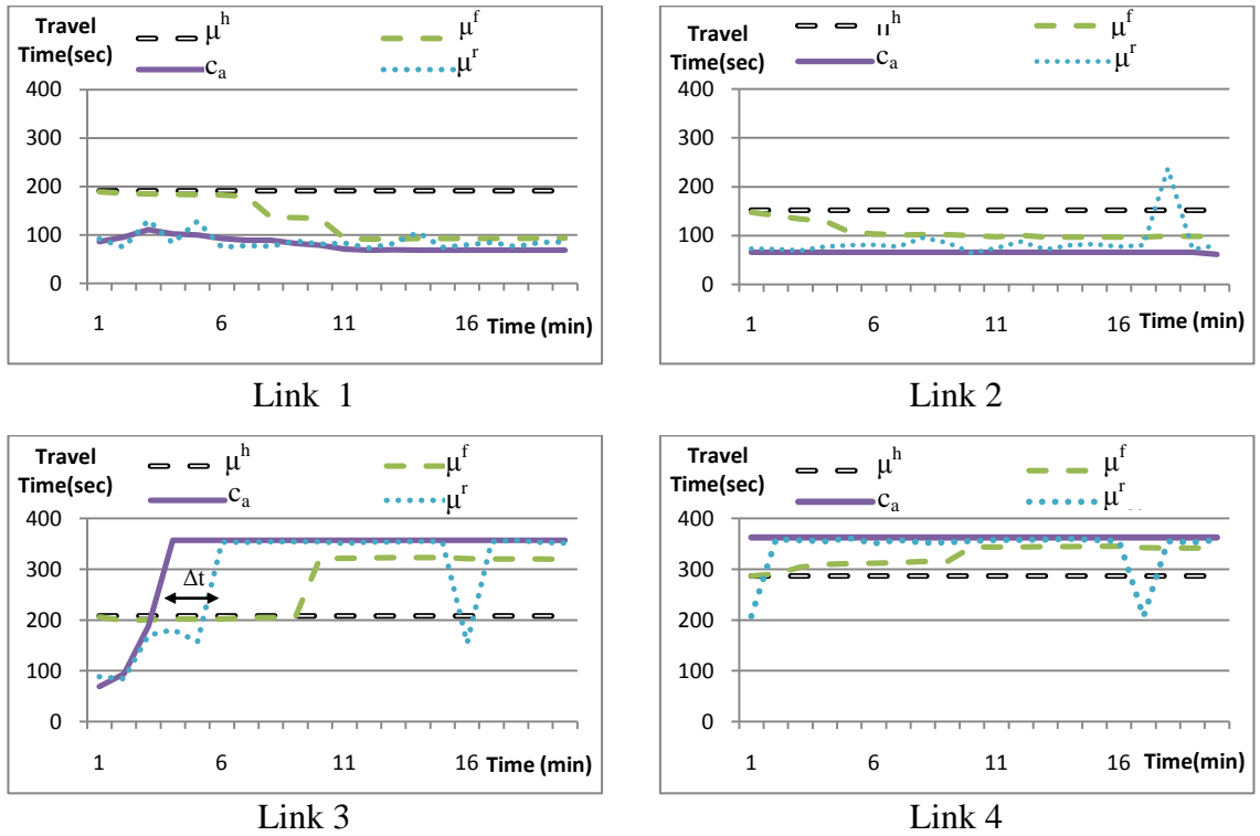
Figure 6.2: Results for information fusion models
